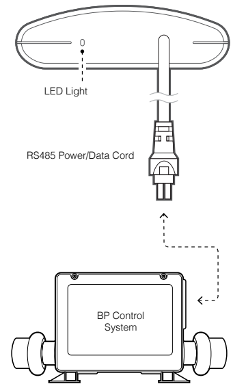
GATEWAY ULTRA Module (side view)
